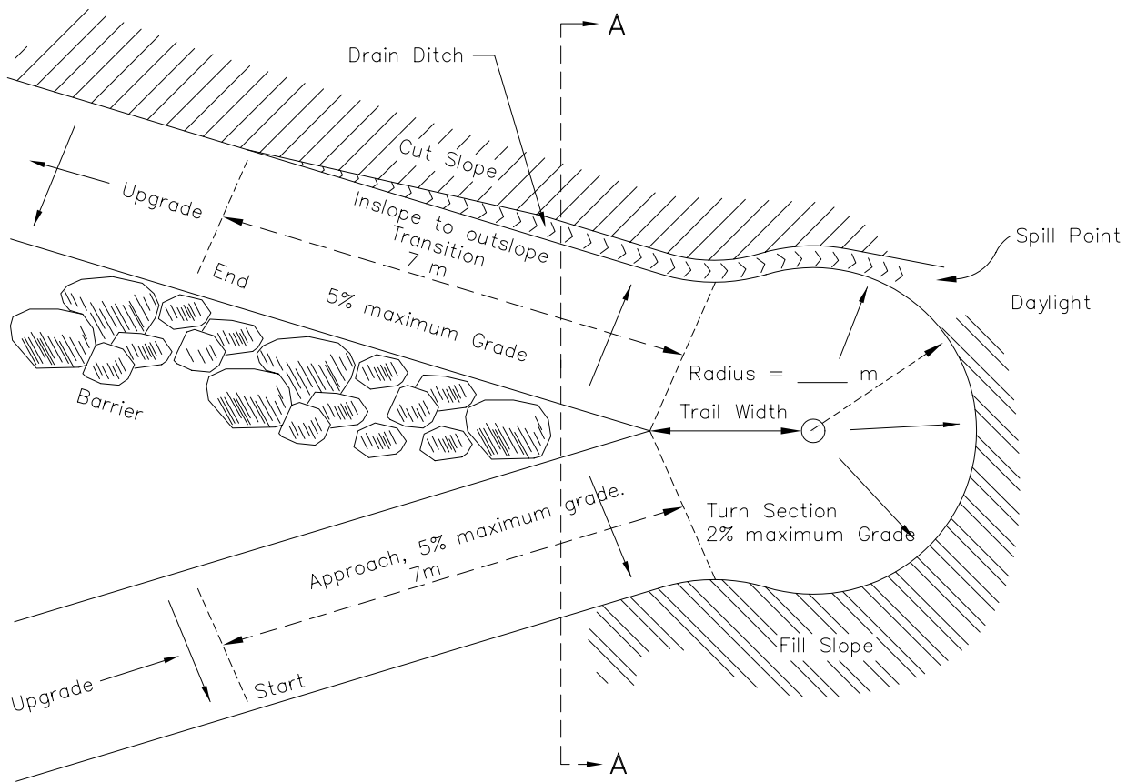
PLAN VIEW
